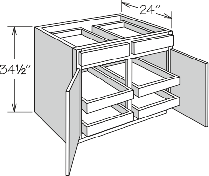
4 SLIDING SHELVES
