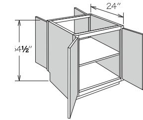
4 BUTT DOORS
