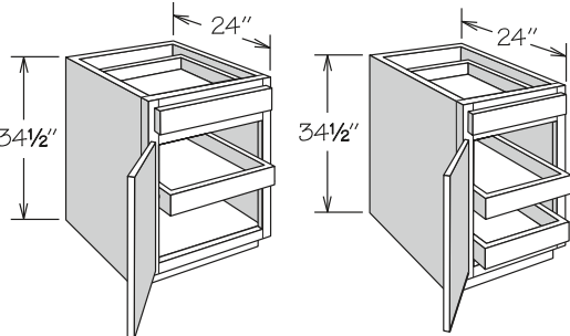
1 SLIDING SHELF
