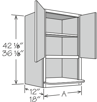
42" High Shown
