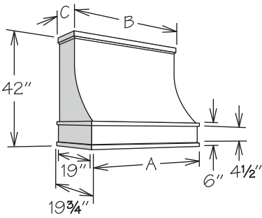
SLOPED __SLWM
