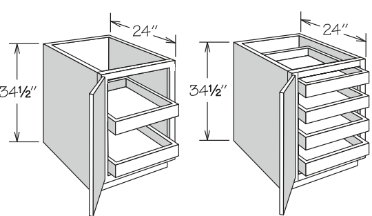
2 SLIDING SHELVES
