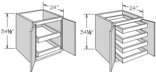
2 SLIDING SHELVES
