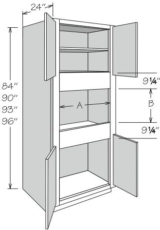
90" High Shown
