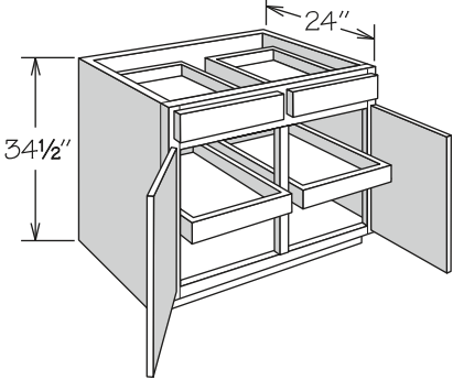
2 SLIDING SHELVES
