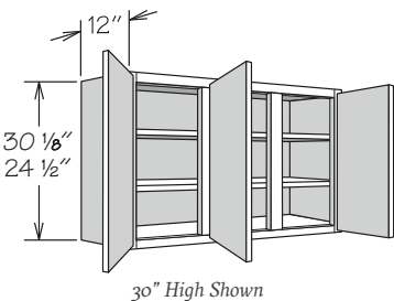
30" High Shown
