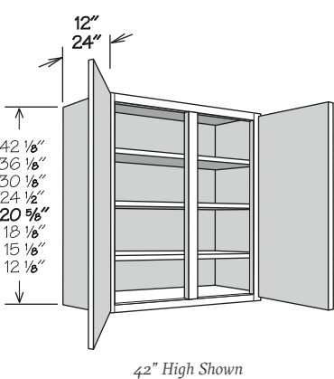
42" High Shown
