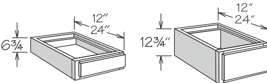
6" HIGH
