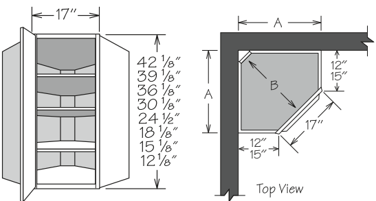
42" High Shown
