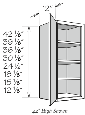
42" High Shown
