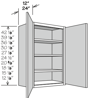
42" High Shown
