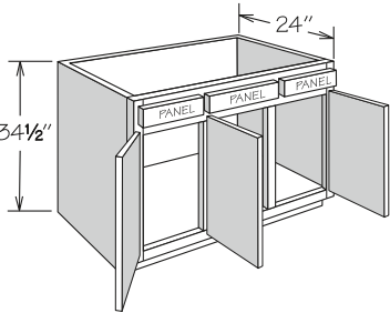
3 DOORS
