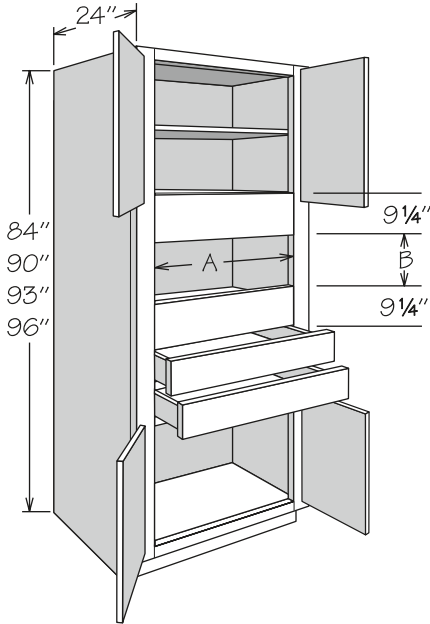
90" High Shown
