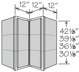
30" High Shown
