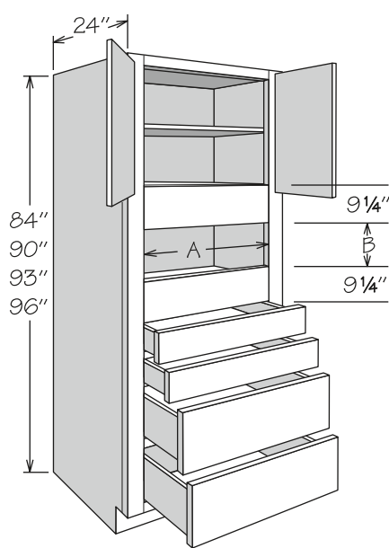
90" High Shown
